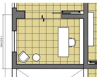
MAIN MASTER BEDROOM EXTENSION AREA. 20.3M2/ 218.5ft2
